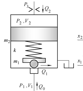
Fig. 6. Modeling of the main stage of pressure relief vae
